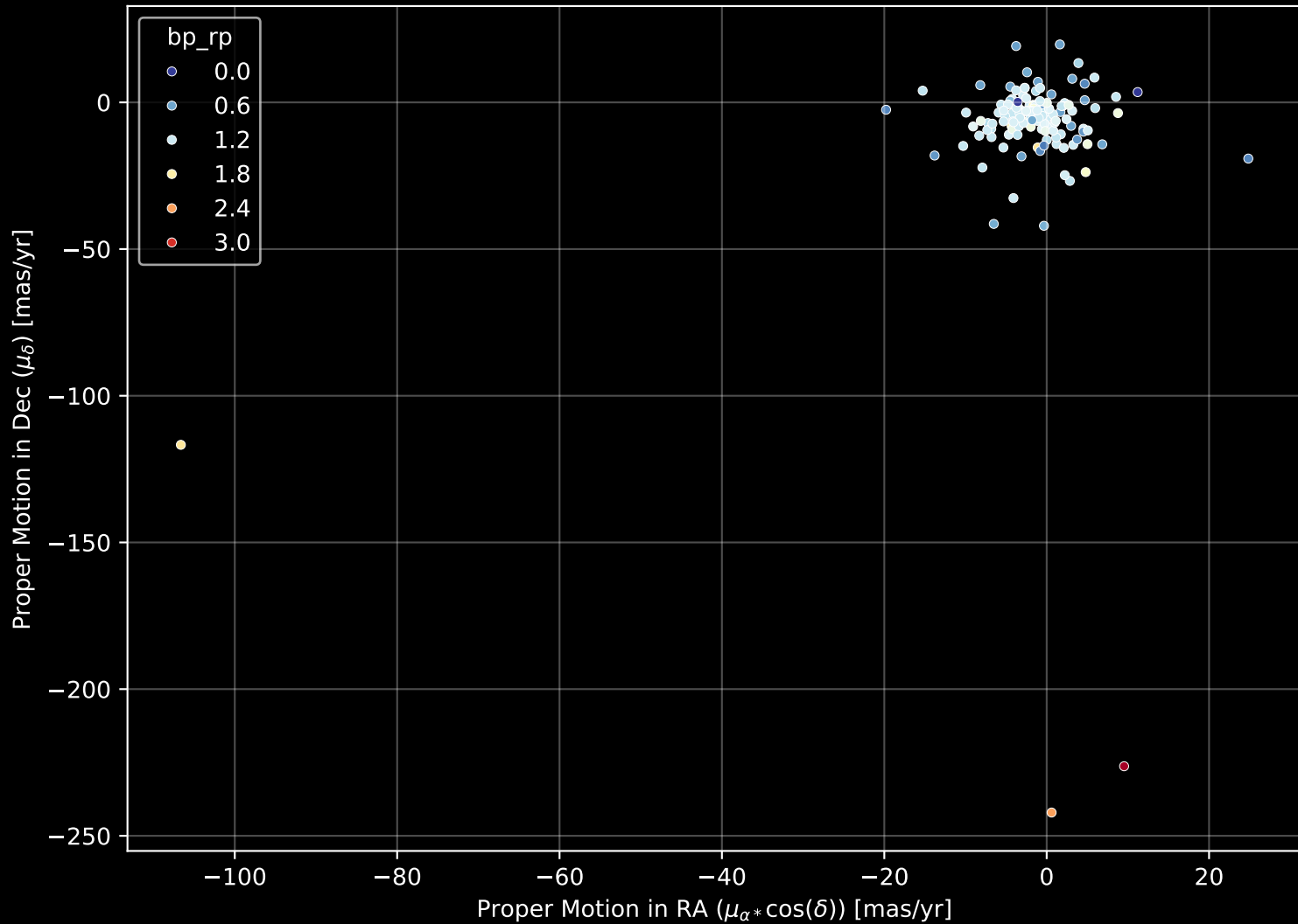
APOGEE DR17 Field: [045+30] Proper Motion Diagram (n= 135)
