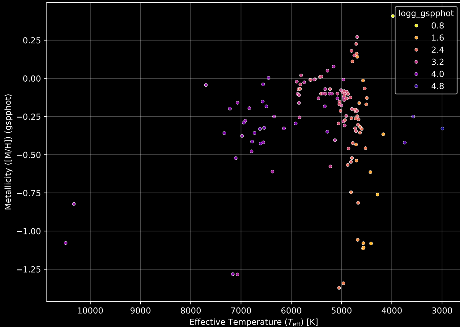
APOGEE DR17 Field: [045+30] Stellar Population Parameters (n= 135)
