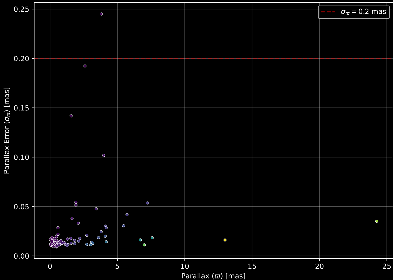
APOGEE DR17 Field: [045+30] Parallax Quality (n= 135)
