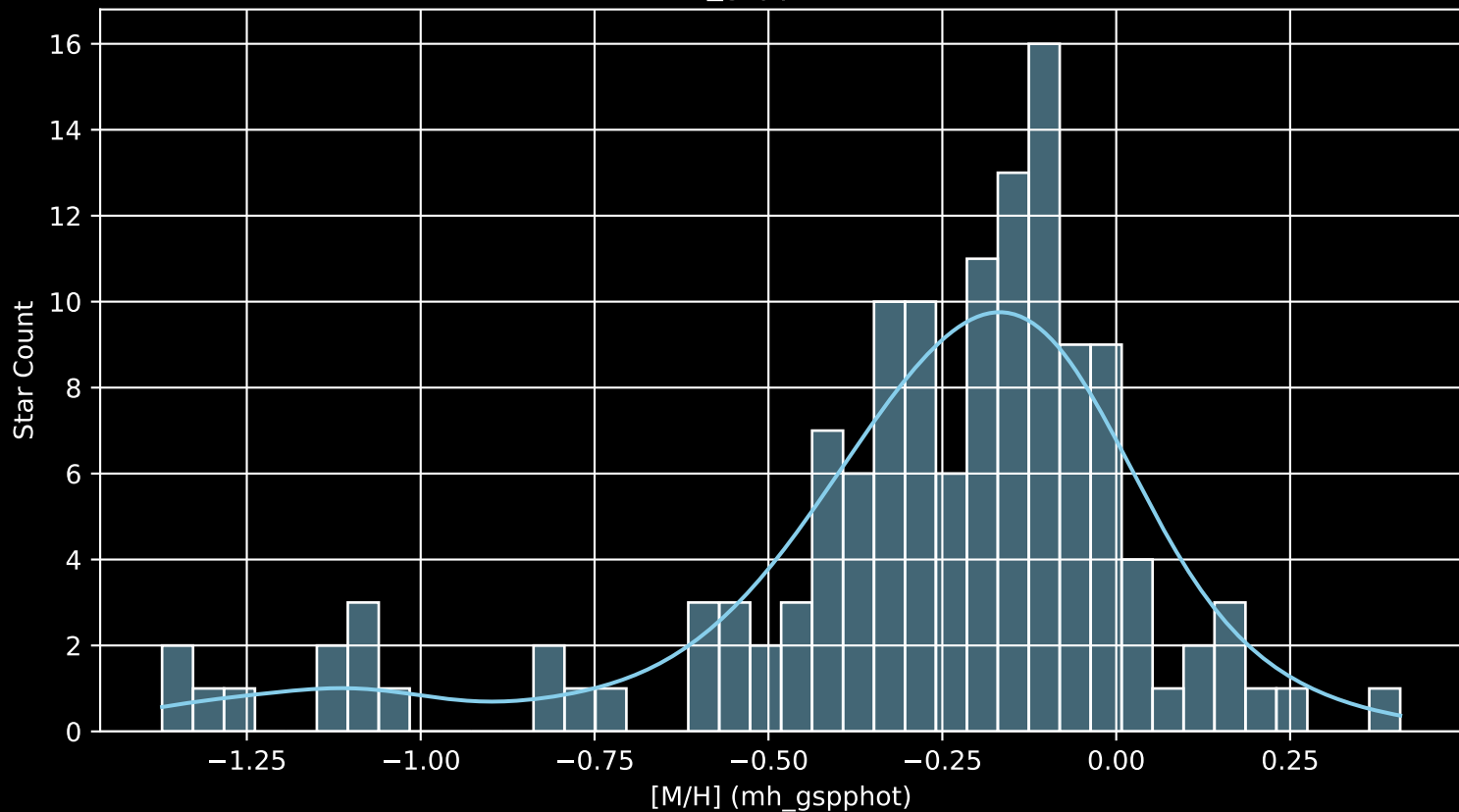
APOGEE DR17 Field: [045+30 [M/H] (mh_gspphot) (n= 135)
