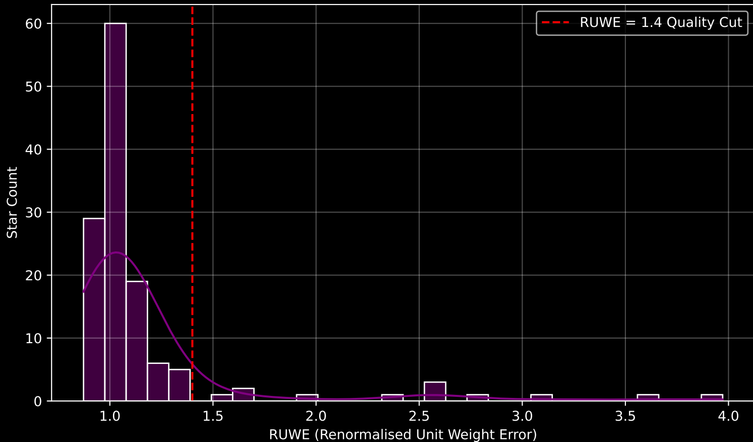
GAPOGEE DR17 Field [045+30] RUWE Distribution (n= 131)
