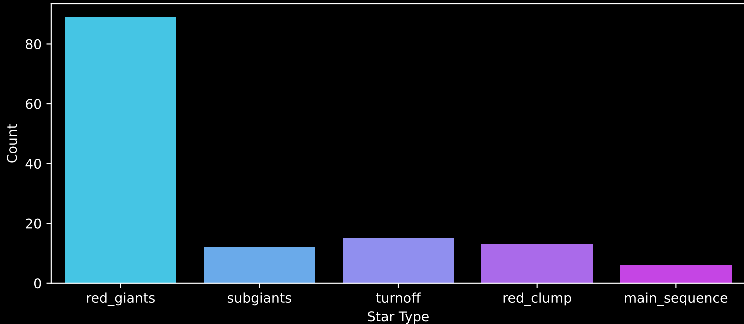
APOGEE DR17 Field: [045+30] Count plot of Star Type
